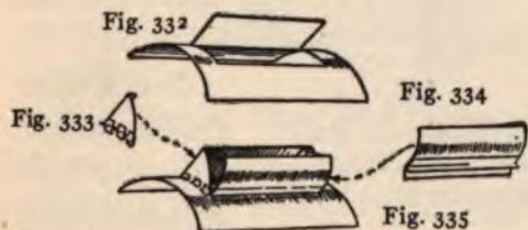
FIG. 332. — Top, showing how Portion is Bent up for Back of Letter-Drop.
